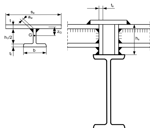
Figure 4. Cross-section of a stiffener and connection to the radial beam The required section modulus is given by
