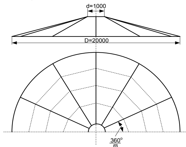
Figure 1. A fixed tank roof
