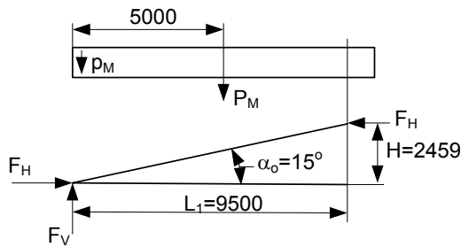
Figure 2. Forces from the roof load
