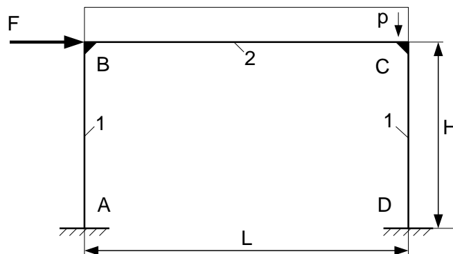
Figure 1. Unbraced planar frame
