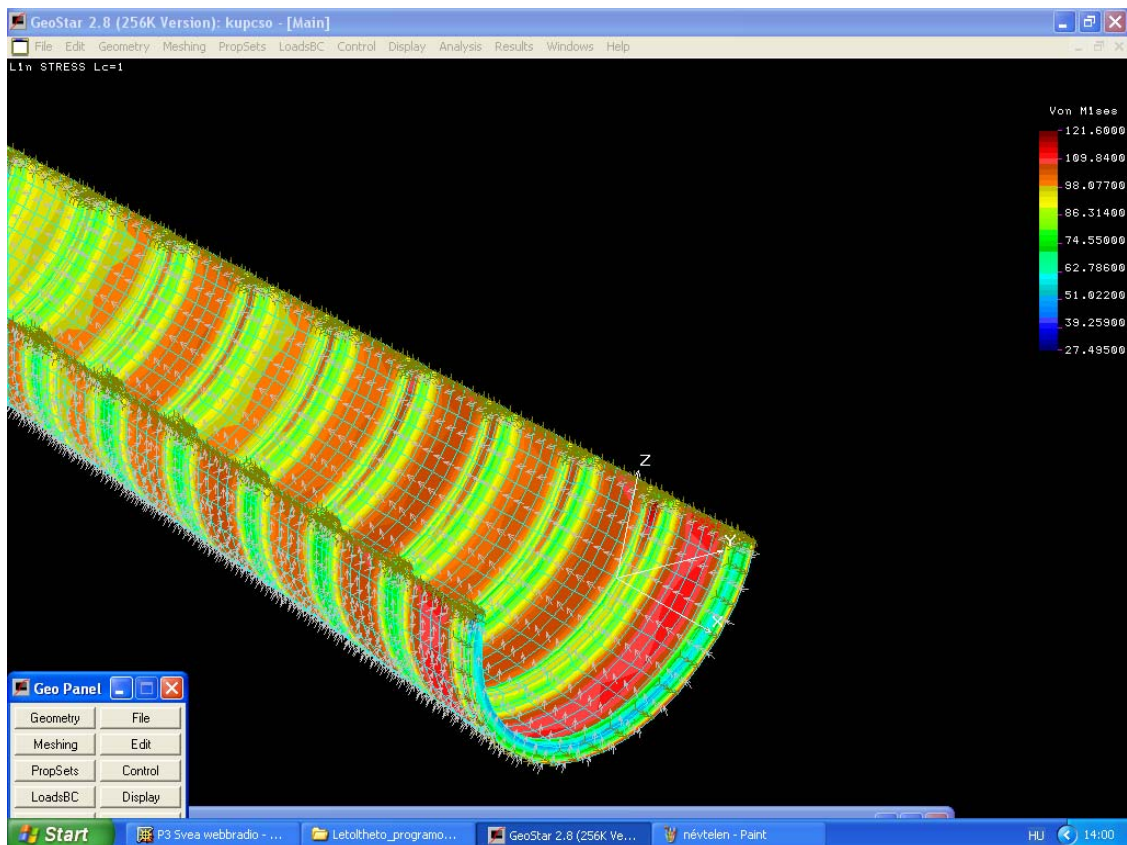
Figure 2. Finite element results of the conical shell stresses
