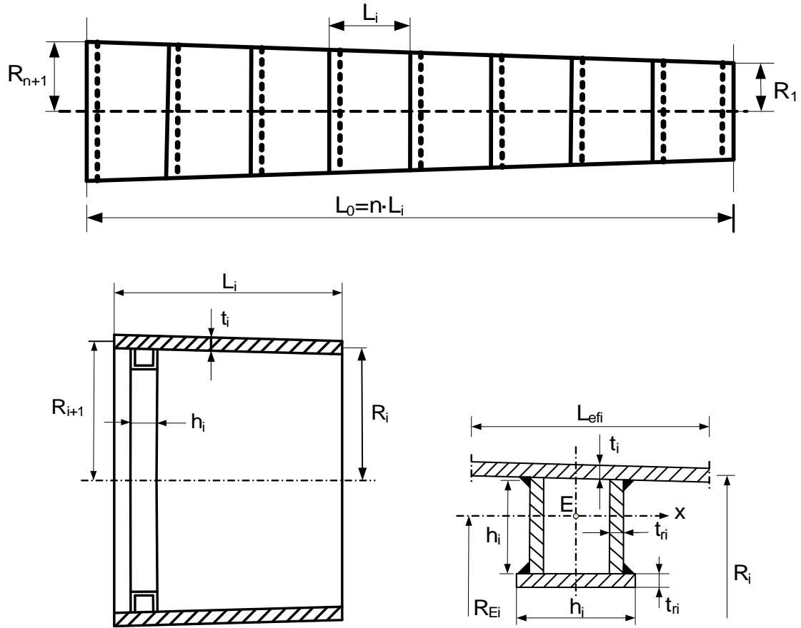
Figure 1. The main dimensions of the conical shell – a shell segment with the ring-stiffener of welded square box section
