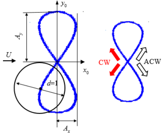
FIGURE 1: LAYOUT FOR FIGURE-EIGHT PATH
