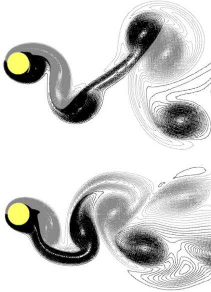
FIGURE 5: VORTICITY CONTOURS FOR CW (TOP) AND ACW (BOTTOM) ORBITS AT TOPMOST CYLINDER POSITION (Re=180; FR=0.85)
