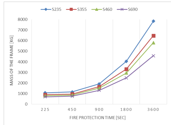
Figure 4. Mass of the frame in case of different types of steel versus fire protection time
