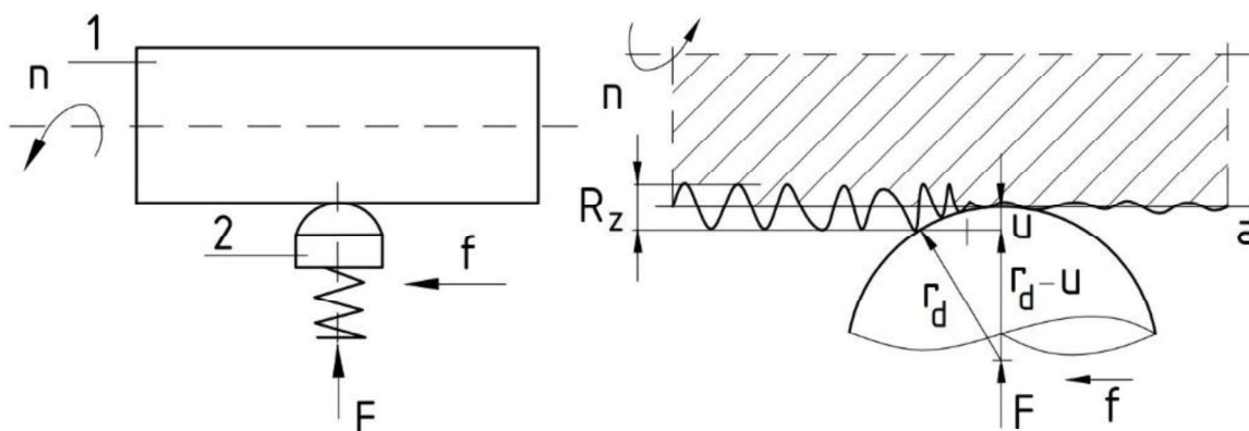
Figure 1 – Kinematics of burnishing [20]
