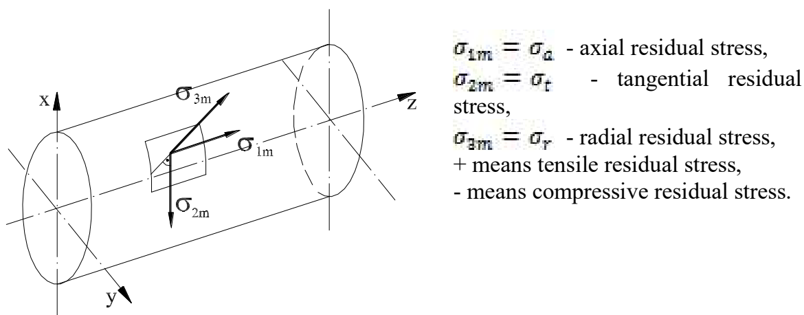
Figure 5 – The main stress direction of cylindrical workpiece [34]
