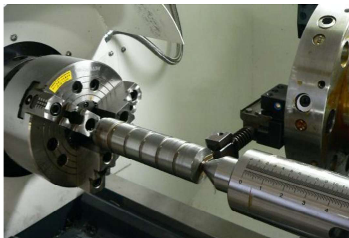
Figure 2 – Burnishing process on OPTIMUM OPTIturn CNC machine
