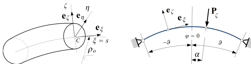
Figure 1: (a) The coordinate system, (b) The centerline with the external load and supports
